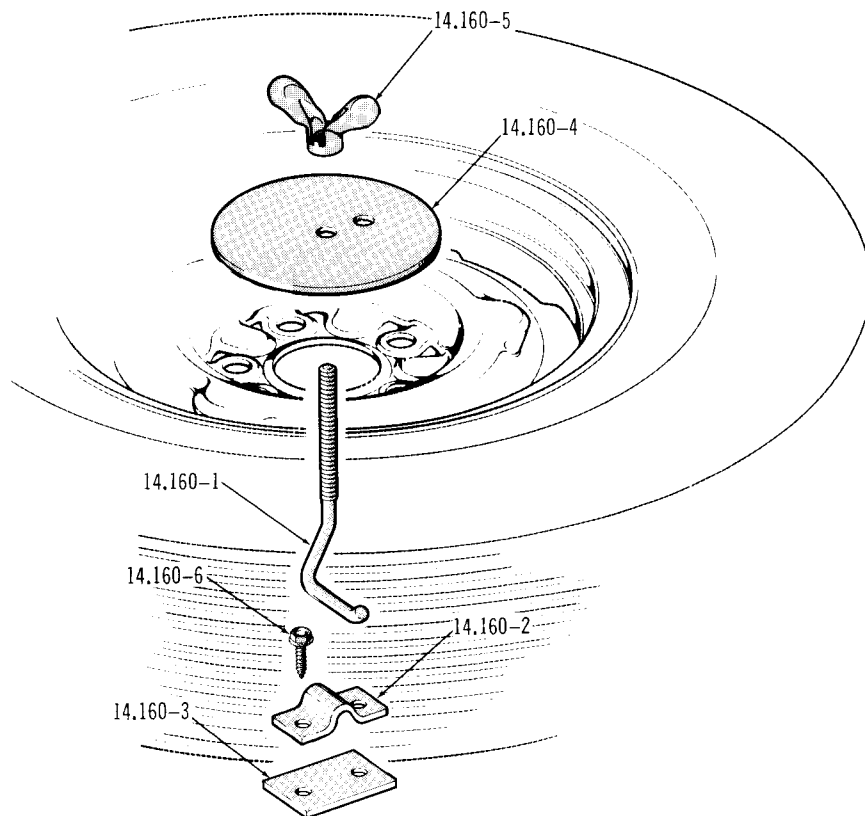
SPARE TIRE REAR FLOOR MOUNTING (INTERIOR) . . . 10
