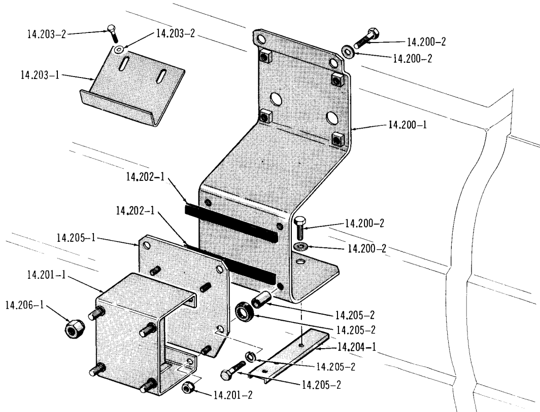
SPARE TIRE MOUNTING (OUTSIDE BOX) . . . 40
