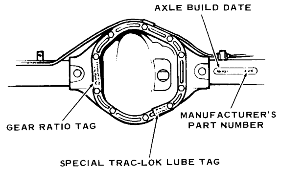
RATIO AND TRAC-LOK DIFFERENTIAL IDENTIFICATION
