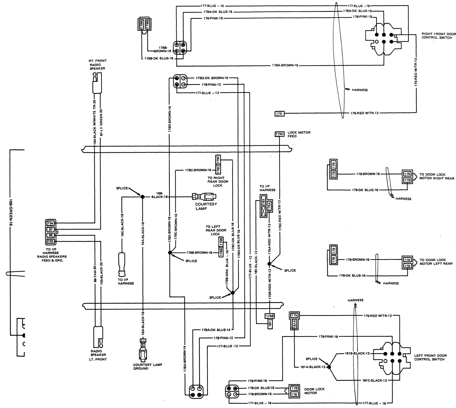
POWER DOOR LOCK DIAGRAM
