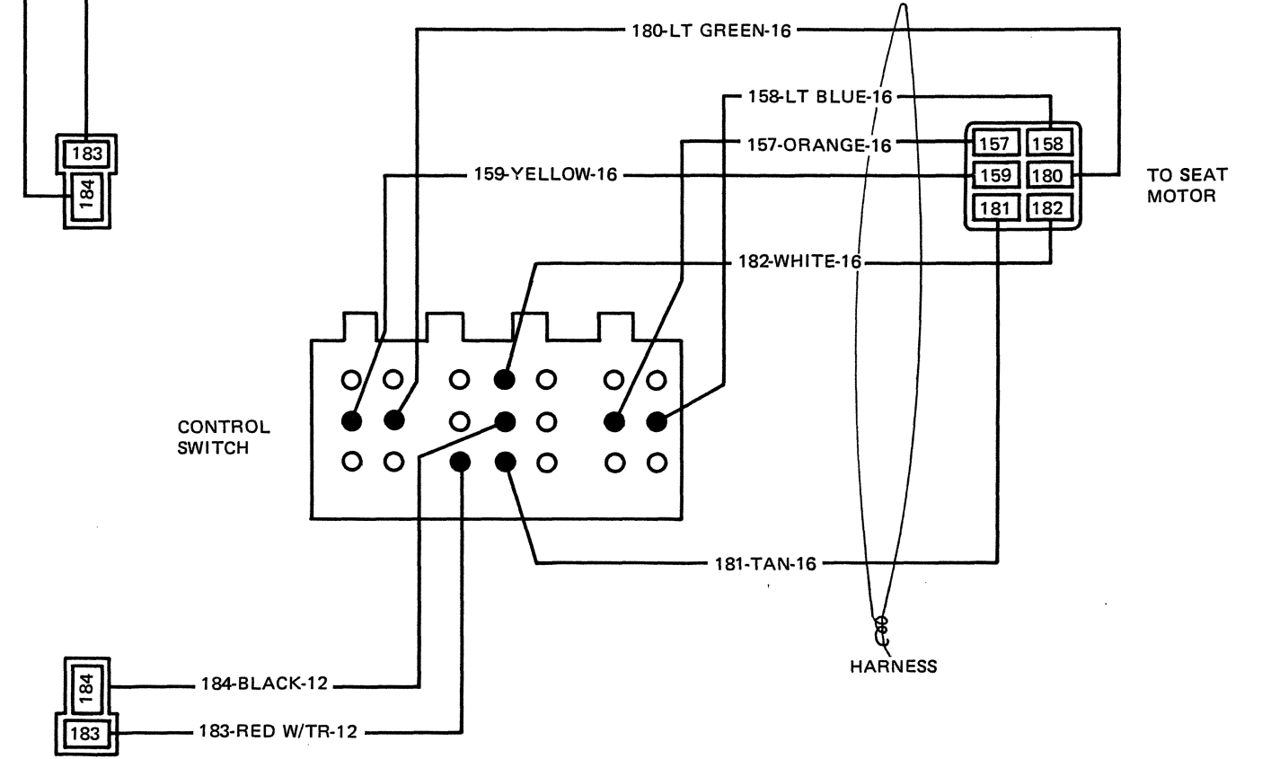
POWER SEAT - DRIVERS SIDE
